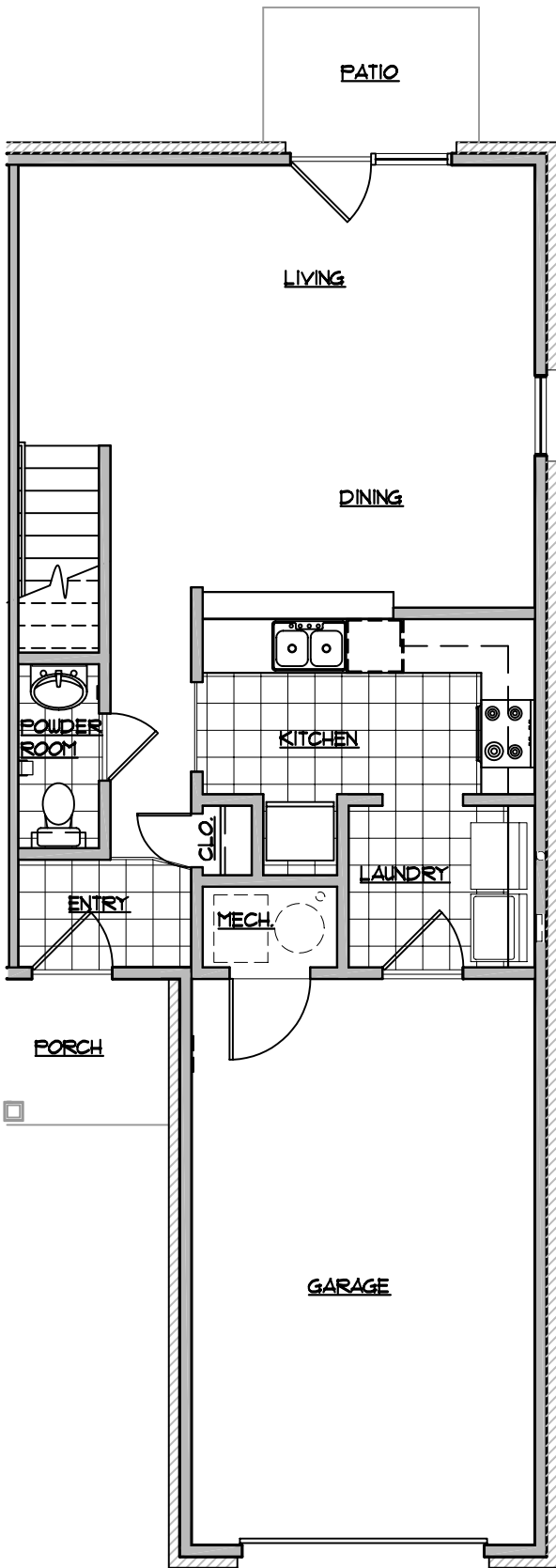
BUILDING TYPE 1 THREE BEDROOM - FIRST FLOOR SCALE: N.T.S.
