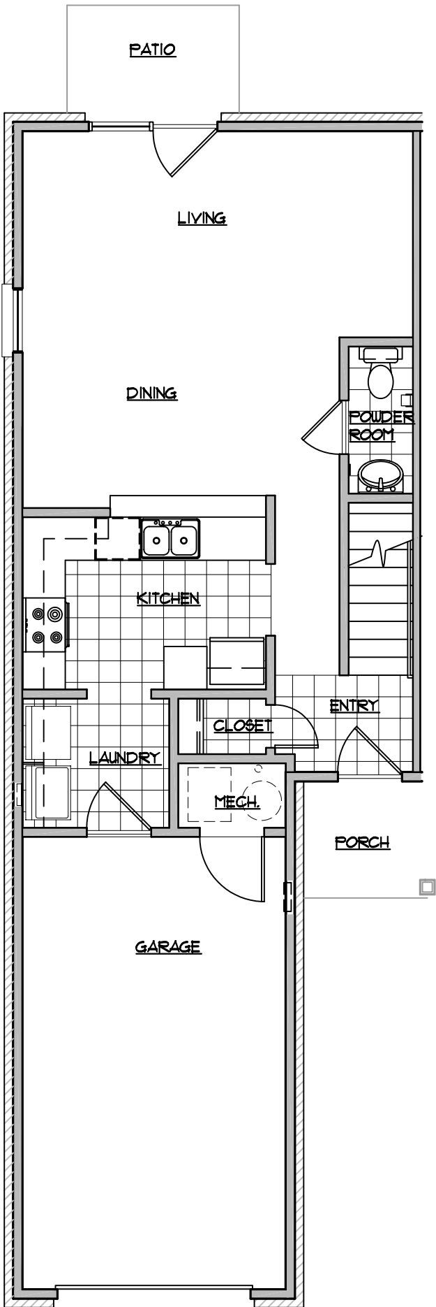
BUILDING TYPE 1 TWO BEDROOM - FIRST FLOOR SCALE: N.T.S.
